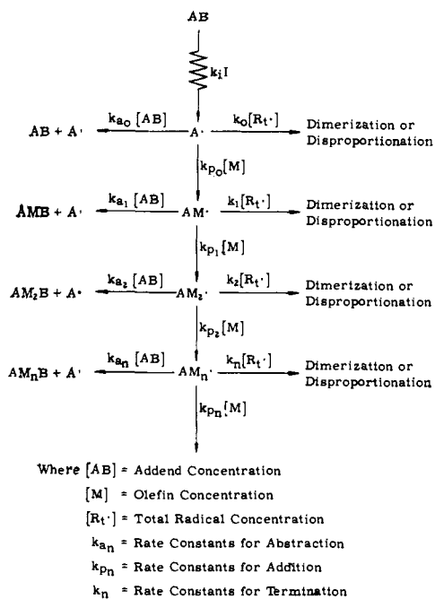
Fig. 1.—Over-all reaction scheme.
