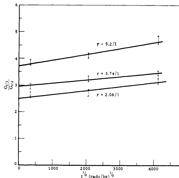
Fig. 6.—Effect of dose rate on G_{11:1}/G_{1:2} for isopropyl alcohol and 1-pentene at 100°.
