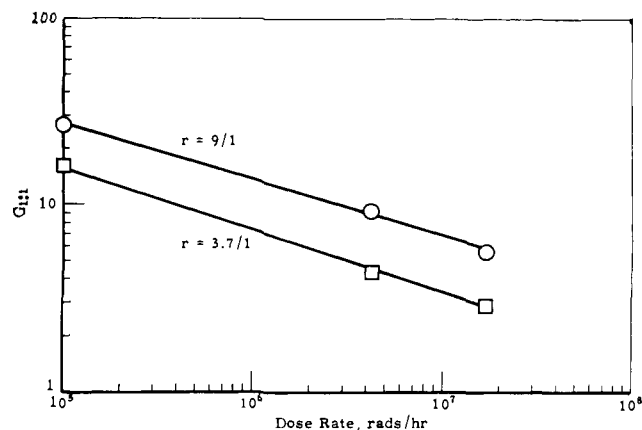
Fig. 2.—Effect of dose rate on G_{1,1} for addition of isopropylamine to 1-pentene at 100^\circ .
