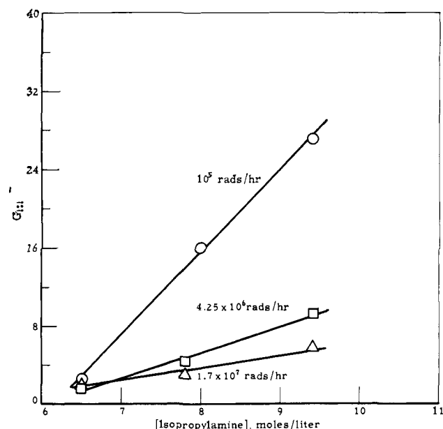
Fig. 3.—Effect of addend concentration on G_{1,1} for addition of isopropylamine to 1-pentene at 100^\circ .
