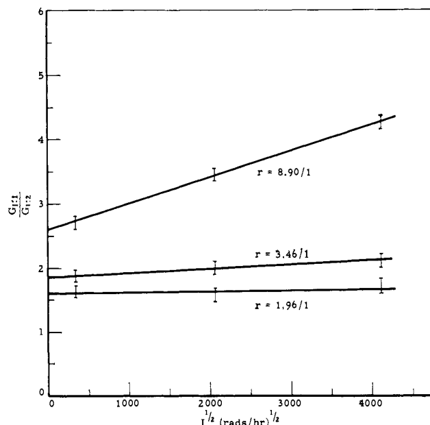
Fig. 5.—Effect of dose rate on G_{11:1}/G_{1:2} for isopropylamine and 1-pentene at 100°.
