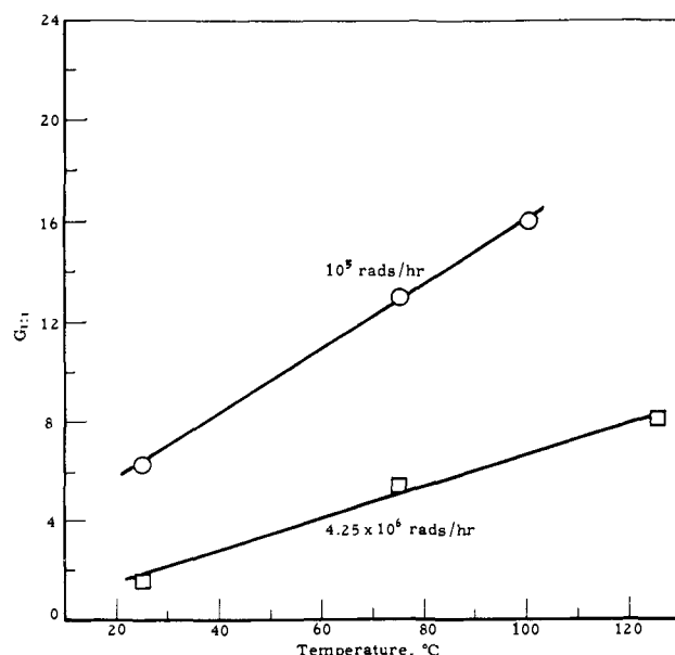
Fig. 4.—Effect of temperature on G_{1,1} for addition of isopropylamine to 1-pentene ( r = 4.0/1 ).
