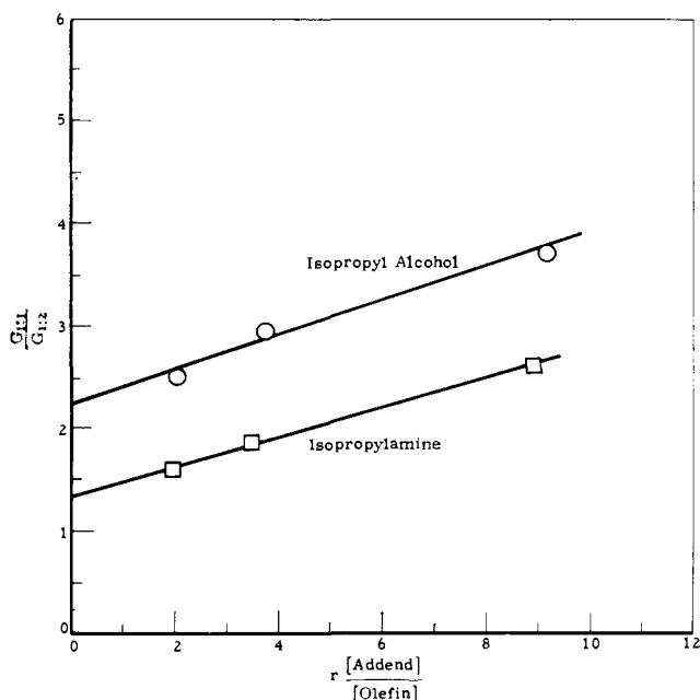
Fig. 7.—Effect of reactant concentration ratio on yield of adducts at zero dose rate.
