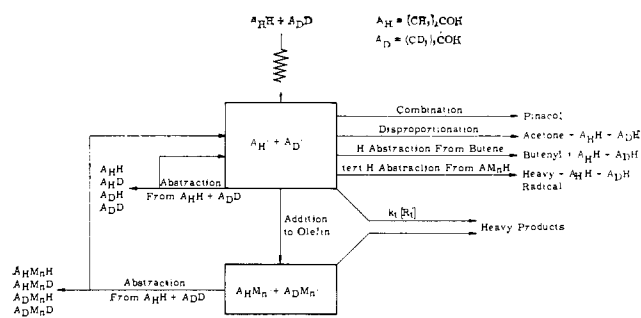
Fig. 8.—Formation and reactions of the isotopic hydroxypropyl radicals.
